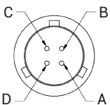
4 PIN Bayonet
