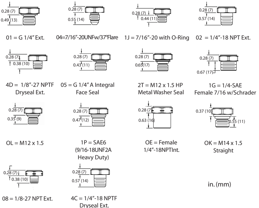
Pressure Fittings Diagram B
